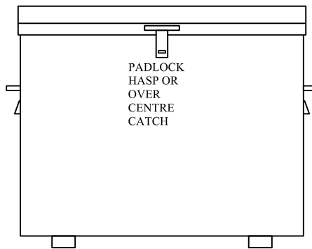
FRONT ELEVATION
